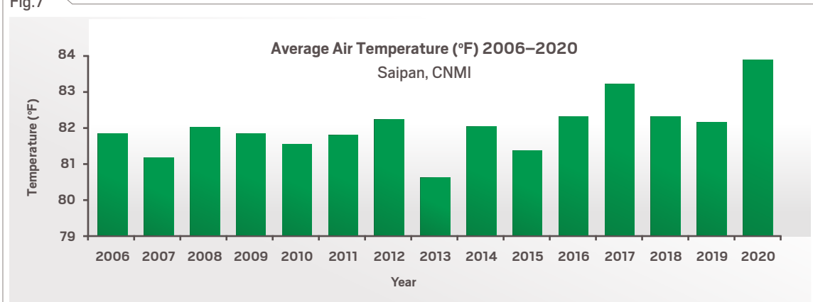
Figure 7. Average annual air temperature from 2006 to 2020 at the Francisco C. Ada Saipan International Airport in the CNMI. Original figure by Abby Frazier, using data from the NOAA GHCN-Daily database (NOAA 2020c; Menne et al. 2012).
