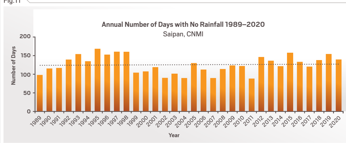
Figure 11. Annual number of days with no rainfall from 1989 to 2020 at Saipan's international airport, CNMI. The black, dotted trend line shows no significant linear trend over time. Original figure by Abby Frazier, using data from the NOAA GHCN-Daily database (NOAA 2020c; Menne et al. 2012).
