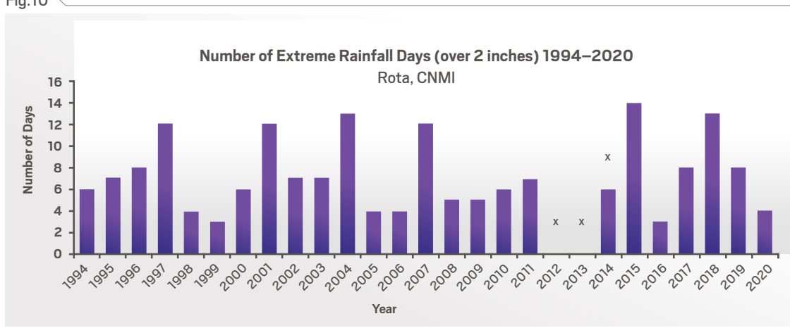
Figure 10. Annual number of days with daily rainfall totals exceeding 2 inches (51 mm) from 1994 to 2020 at Rota's international airport. The asterisks (*) represent years in which significant data were missing. Original figure by Abby Frazier, using data from the NOAA GHCN-Daily database (NOAA 2020c; Menne et al. 2012).
