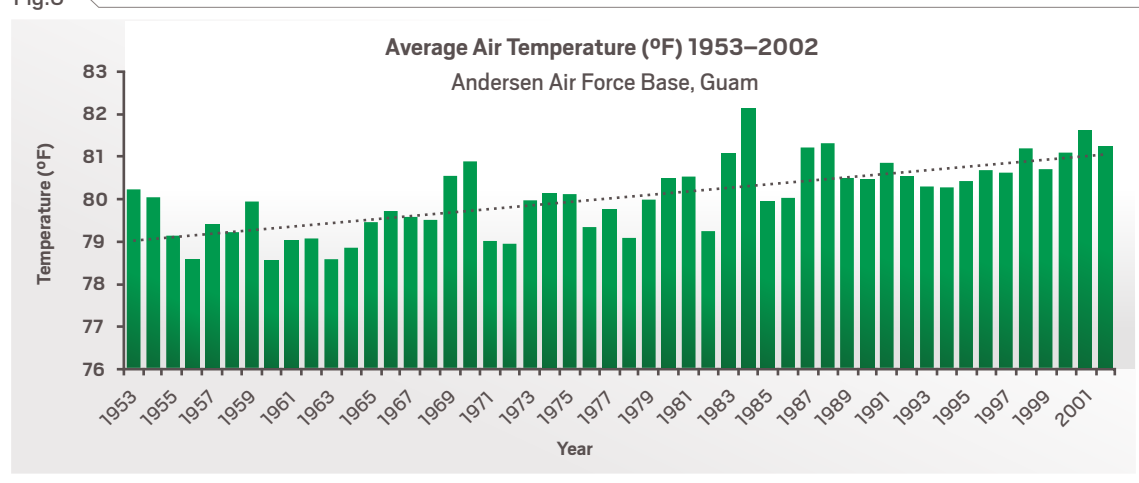
Figure 6. Average annual air temperature at Andersen Air Force Base in Guam 1953–2002. The long-term linear trend indicated by the black, dotted line shows an increase over time. Original figure by Abby Frazier, using data from the NOAA GHCN-Daily database for 1953–2002 (NOAA 2020c; Menne et al. 2012).
