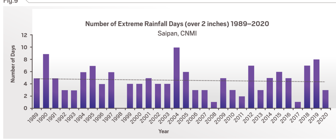
Figure 9. Annual number of extreme rainfall days, with daily rainfall totals exceeding the 99th percentile of the distribution (approximately 2 inches, or 51 mm) from 1989 to 2020 at the Francisco C. Ada Saipan International Airport. The linear trend line (black, dotted line) shows no significant change over the record. Original figure by Abby Frazier, using data from the NOAA GHCN–Daily database (NOAA 2020c; Menne et al. 2012).
