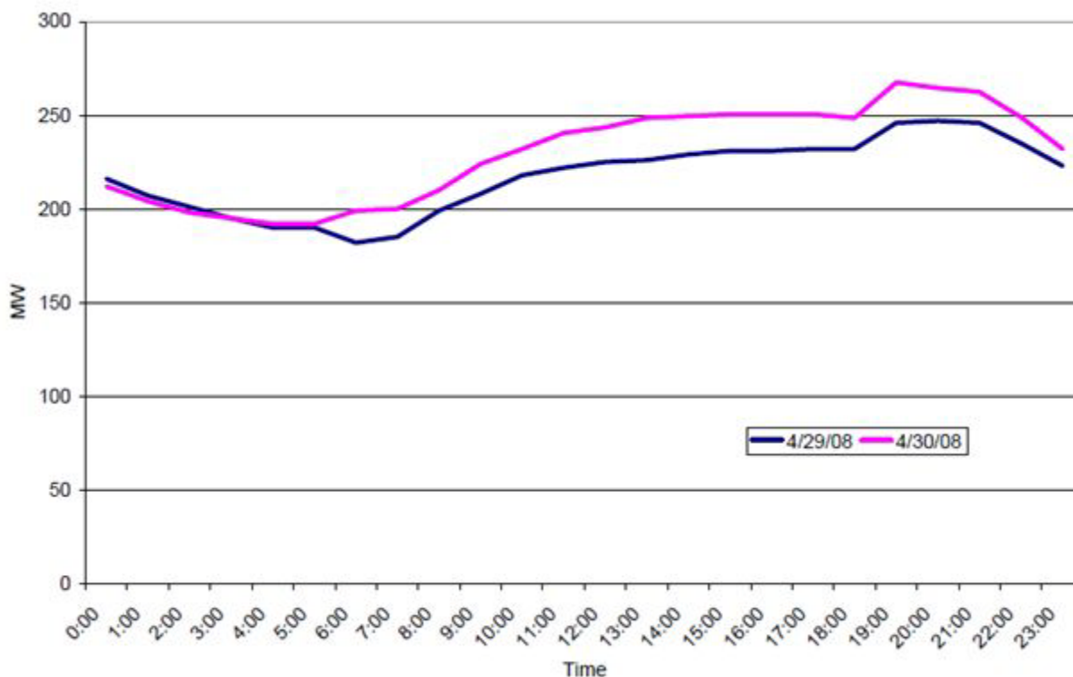
Figure 27. GPA average hourly generation requirements
