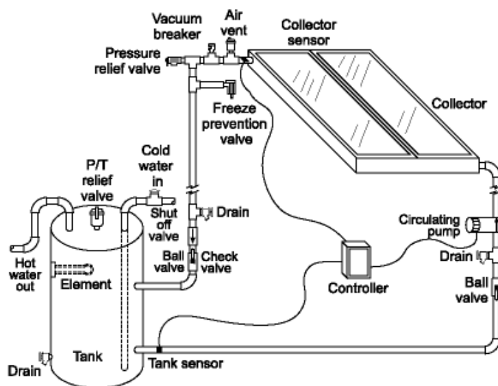
Figure 20. A common solar thermal system
